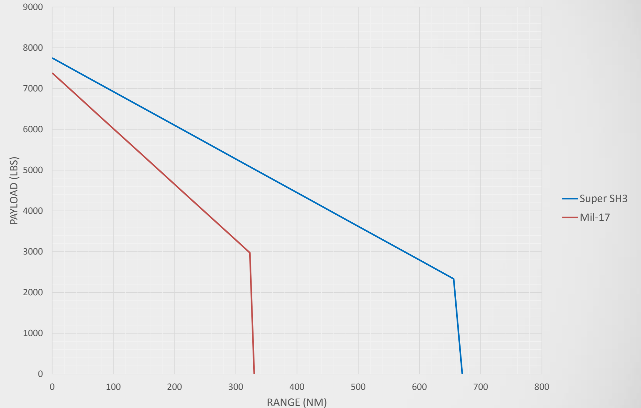
Troop Transport Mission Performance 6000 Ft 30 C
